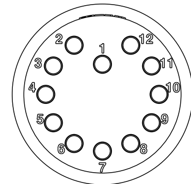
Pin Assignment(Front View)
