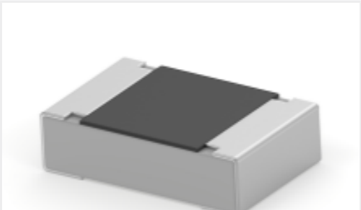
TE Part #3-2176342-5 CRGCQ 0805 470K 5%
