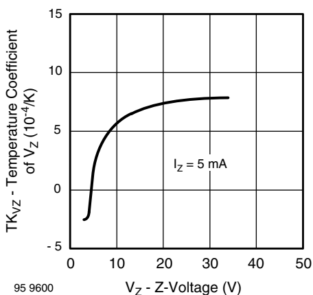
Fig. 2 - Typical Temperature Coefficient of V_Z vs. Z-Voltage
