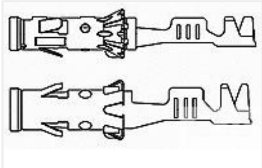
TE Part #929974-8 2,5MM ST-KONT EDS
