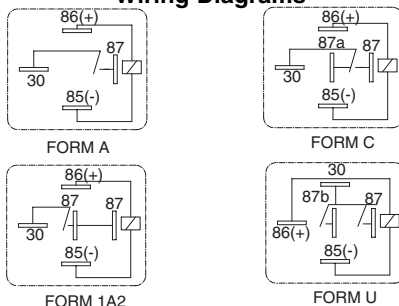
Viewed Toward Terminals
