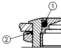
K - (1) Internal seal & (2) front panel seals meet IP65
