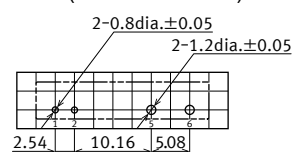
Recommended PC board pattern (BOTTOM VIEW)
