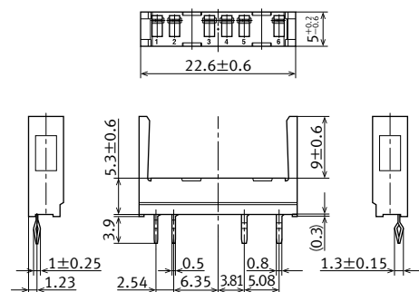
External dimensions
