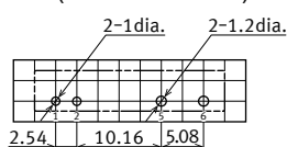
Recommended PC board pattern (BOTTOM VIEW)
