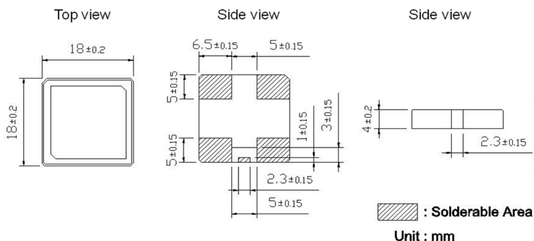
Fig. I Mechanical Data
