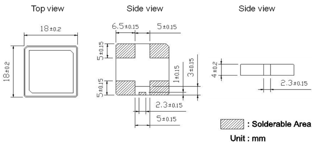
Fig. 1 Mechanical Data
