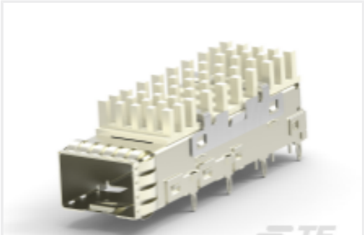
TE Part #2291634-2 SFP+ 1X1 CAGE ASSY, PF,WITH HEATSINK
