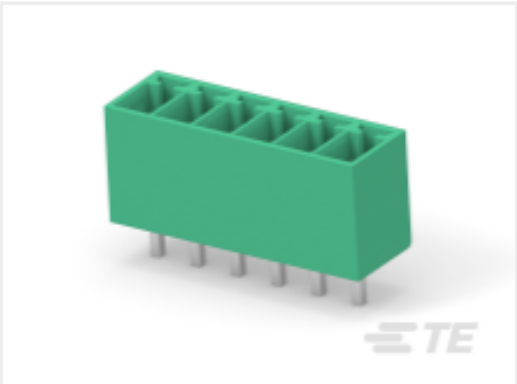
TE Part #2351886-6 6POS TB HDR 180 DEG, PITCH 3.5, TL 3.4mm
