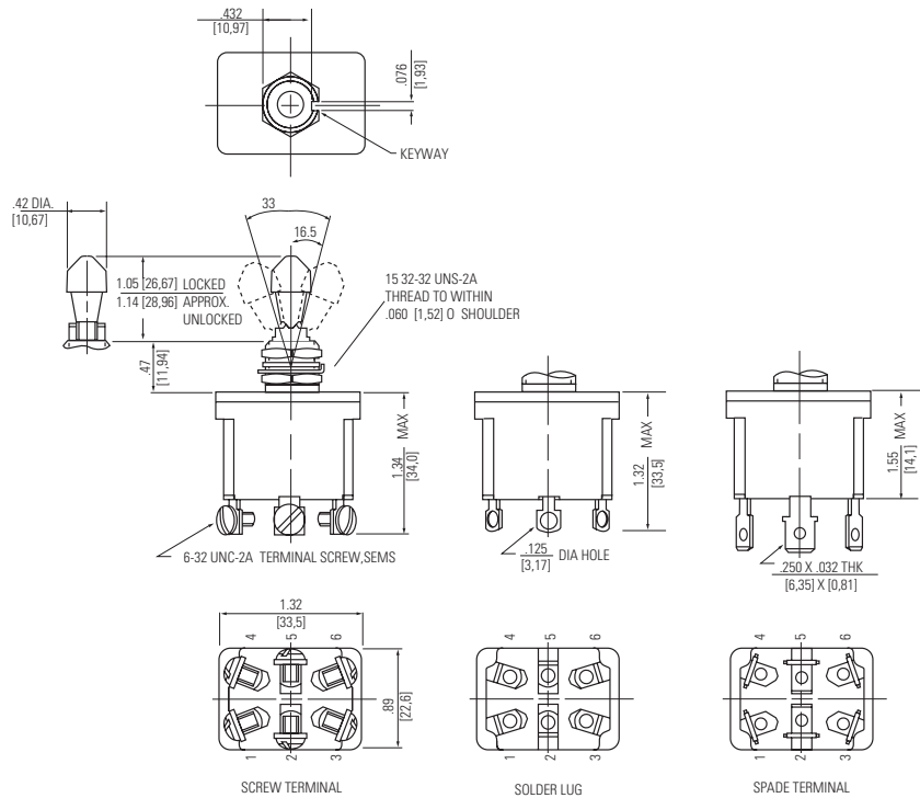
Terminal Identification
