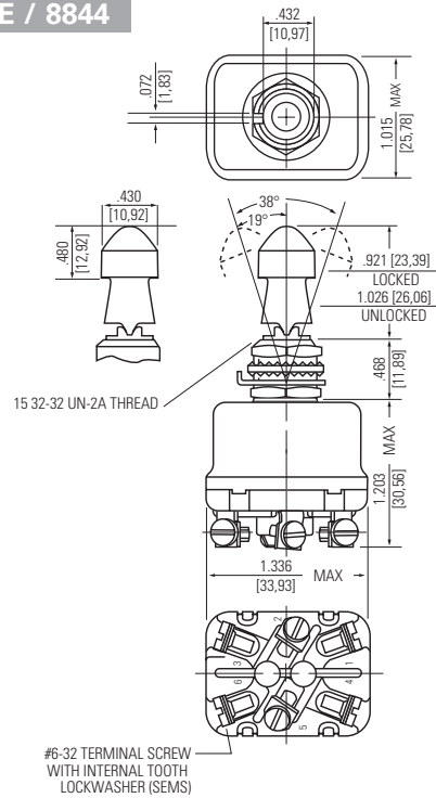
Terminal Identification
