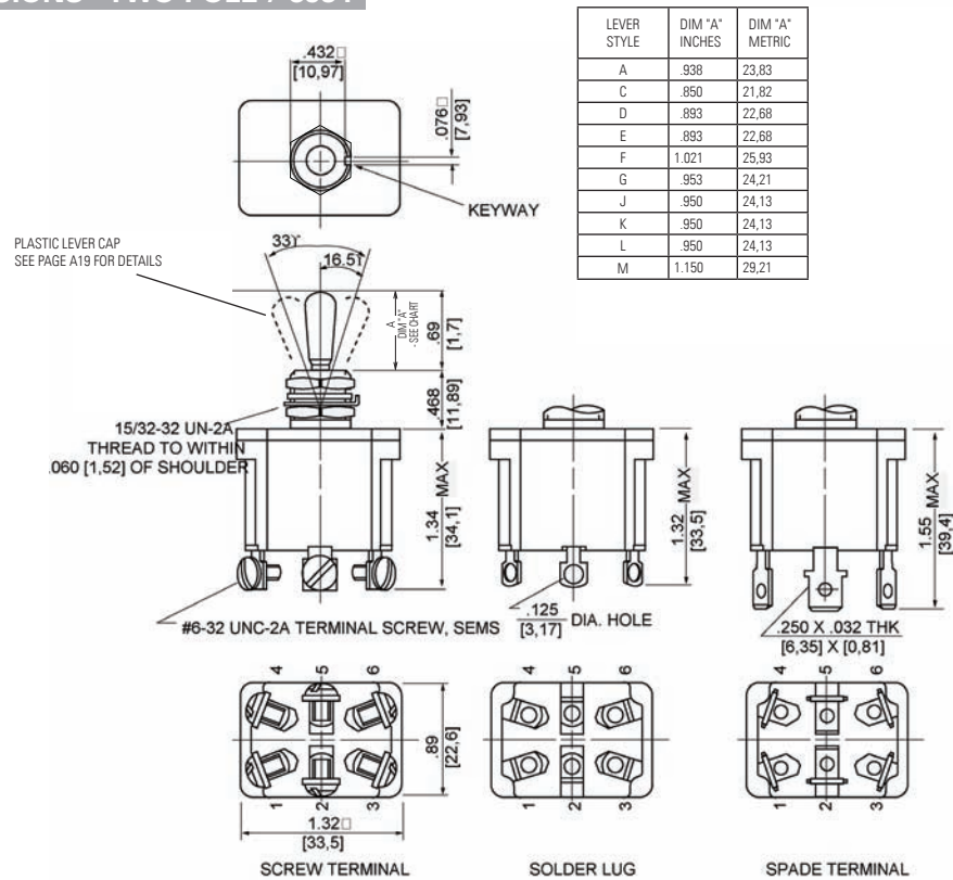
Terminal Identification
