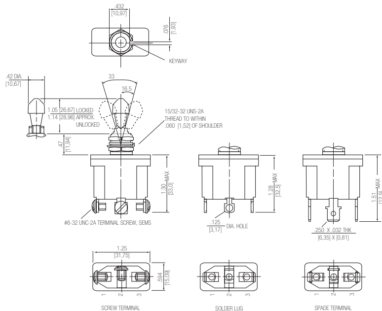
Terminal Identification
