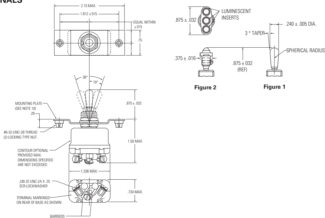
Terminal Identification
