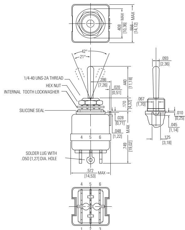
Terminal Identification
