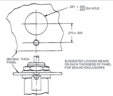
Figures A thru L do not represent details of construction. They schematically illustrate locking function.
