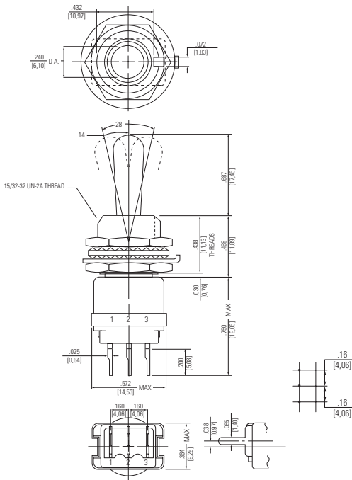
8868 Straight PC Mount
