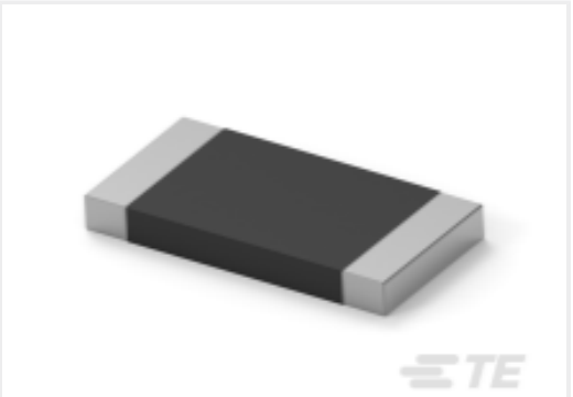
TE Part #6-2176422-4 TLRP 2512 3.0W R039 1% 50PPM 4K RL
