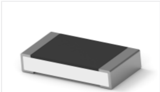
TE Part #6-2176389-0 RQ 1206 442R 0.1% 10PPM 5K RL
