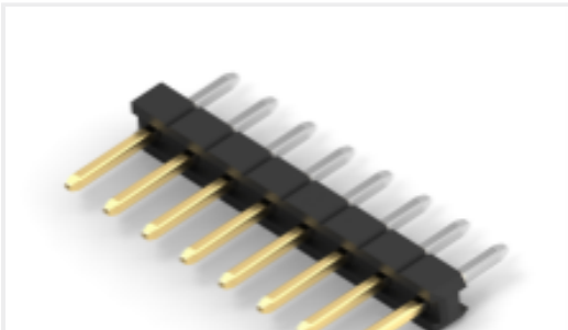
TE Part #2355172-8 8P,2MM,BRK HDR,SRVT,2.8,0.1AU,BOX
