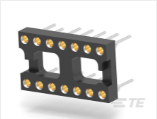
TE Part #CAT-D625-80007 DIP Socket: Standard, Stamped & Formed, Open, Gold
