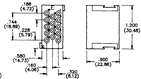
SOCKET HOUSING 765-19-0080E (without contacts)
