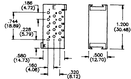
PIN HOUSING 765-14-0080E (without contacts)
