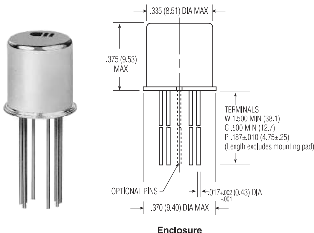
Enclosure
