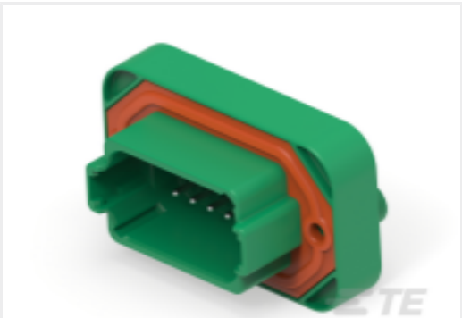
TE Part #DT15-12PC HDR, 12P, GRN, ST, NI/CU, C
