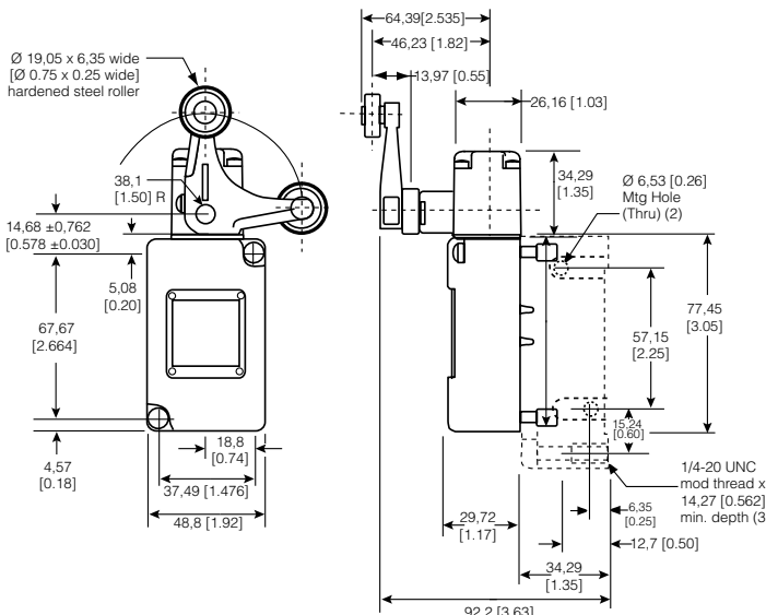
Figure 19. 206LS1 Dimensions
