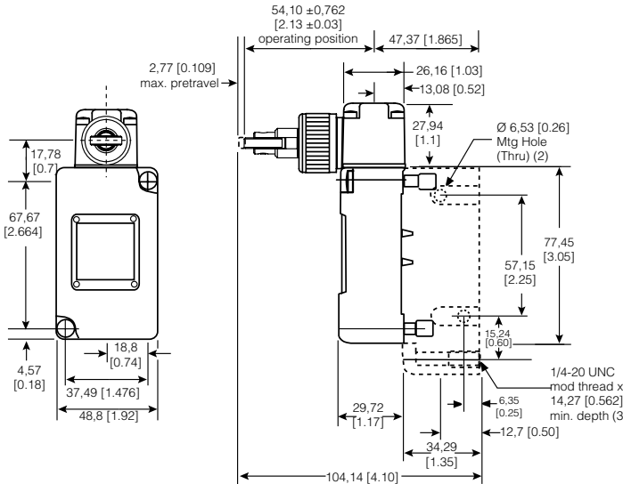
Figure 16. 203LS1 Dimensions
