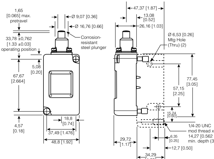
Figure 16. 203LS1 Dimensions
