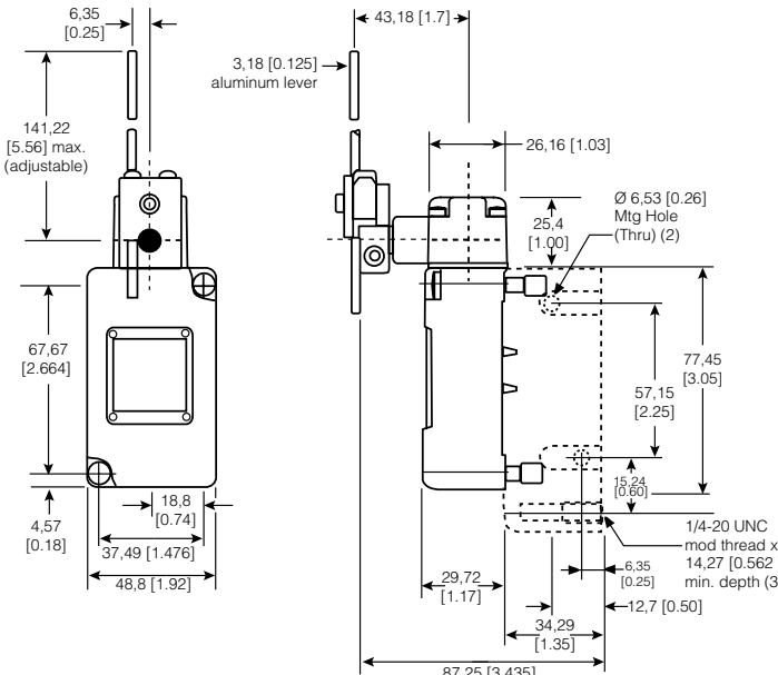
Figure 15. 202LS1 Dimensions
