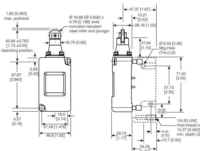
Figure 19. 206LS1 Dimensions
