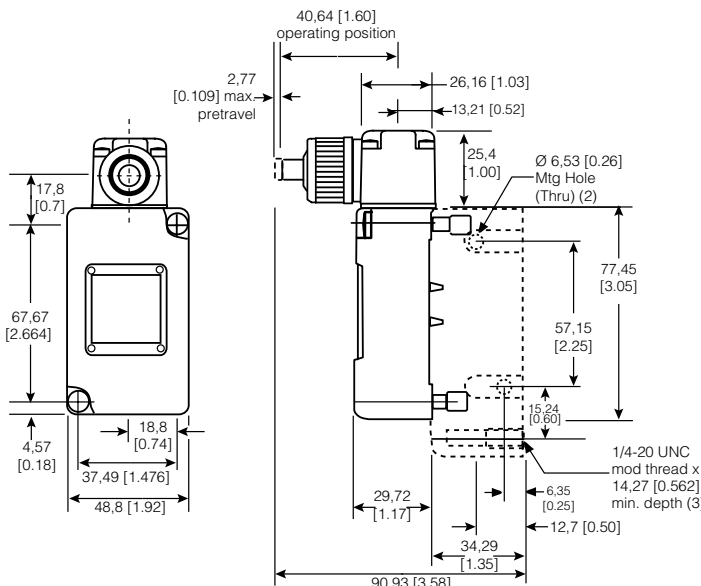
Figure 18. 205LS1 Dimensions
