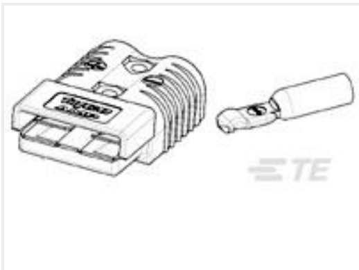
TE Part #1604042-4 KIT,175A,1/0 AWG,GRAY
