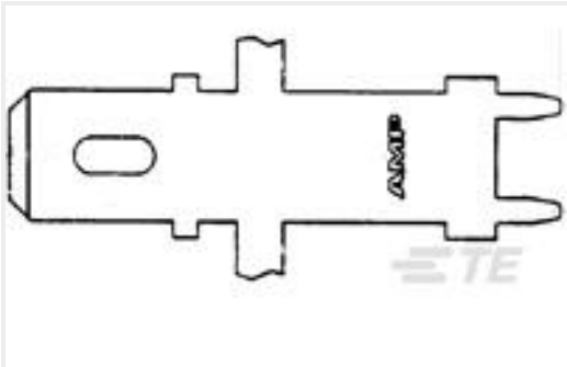
TE Part #63950-1 250 FASTON TAB TPBR
