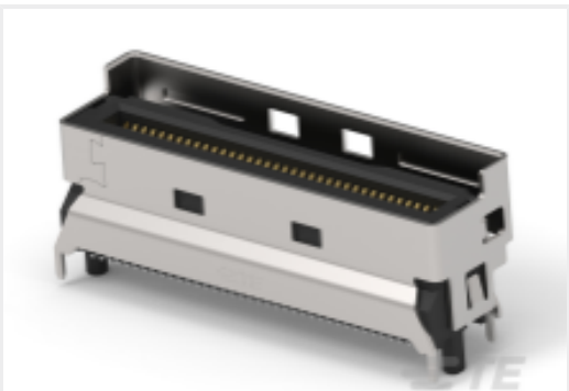
TE Part #2379397-6 MCIO INTERGRATED CONN, V/T,8X, SMT TYPE
