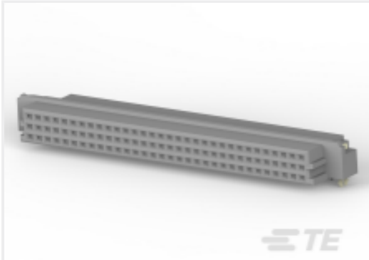
TE Part # 5650897-5 ASSY, RECEPT, EURO, TYPE R, L-FREE, A&C, 64/96
