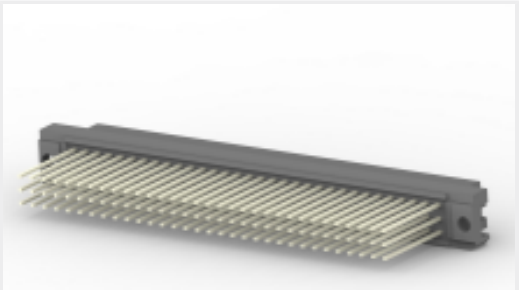
TE Part # 5536366-5 ASSY,PIN,EURO,TYPE C,LEAD-FREE, 96 POS.,,
