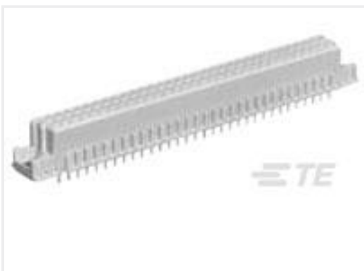
TE Part # 2-1393640-4 V42254B2102C960=PC612 FEDERLEI
