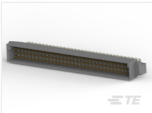
TE Part # 5650473-5 ASSY,PIN,EUROCARD,TYPE C,LEAD-FREE,96,18
