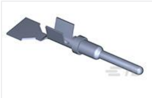
TE Part #638112-1 PIN, SF, SIZE 16, 14-18 AWG,NO INS, AU/SN
