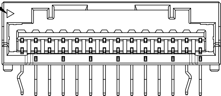
12~15極 12-15 CIRCUITS
