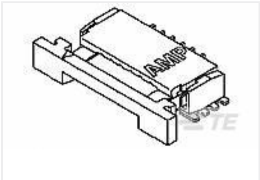
TE Part #2-84952-0 1MM FPC HORZ.BTMM CONT.ASS.20P
