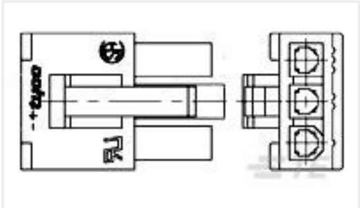
TE Part #1-480701-2 03P UMNL CAP HSG RED
