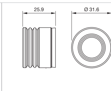
Dimensions [mm] for Part No. 45-545.1K00
