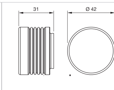
Dimensions [mm] for Part No. 45-543.1K00
