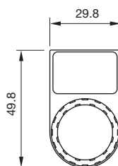
Dimensions [mm] for Part No. 45-567.1103
