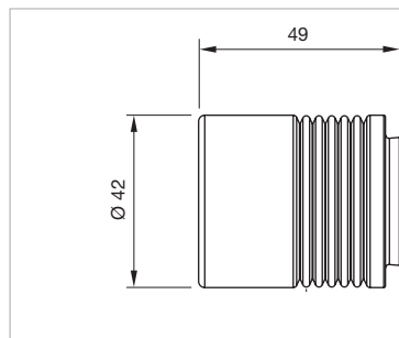
Dimensions [mm] for Part No. 45-542.1K00
