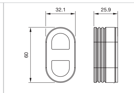
Dimensions [mm] for Part No. 45-547.1K00, 45-548.1K00
