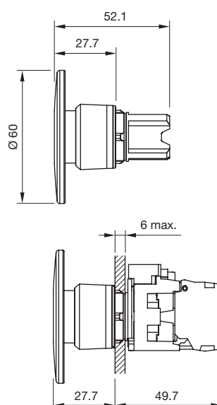
Mushroom-head pushbutton Ø 60 mm (raised design)
