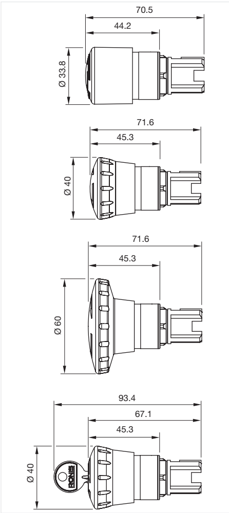
Dimensions [mm]
