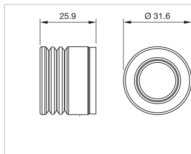
Dimensions [mm] for Part No. 45-544.1K00
