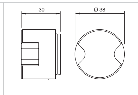
Dimensions [mm] for Part No. 45-546.1K00
