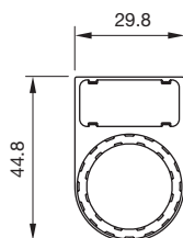
Dimensions [mm] for Part No. 45-567.1103
