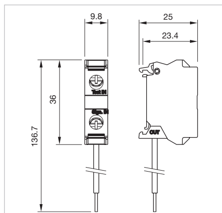
Dimensions [mm]
