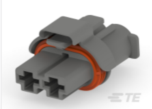
TE Part #1544361-3 2 W 8MM NG2 REC.ASS.GREY
