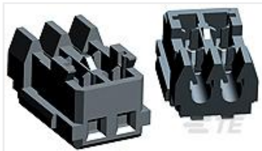
TE Part # 2-292271-0 MT REC ASSY AU-PL. 20P GRAY
