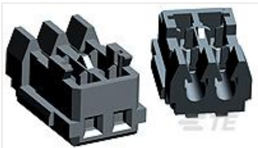
TE Part # 6-292271-9 MT REC ASSY AU-PL. 19P BLUE
