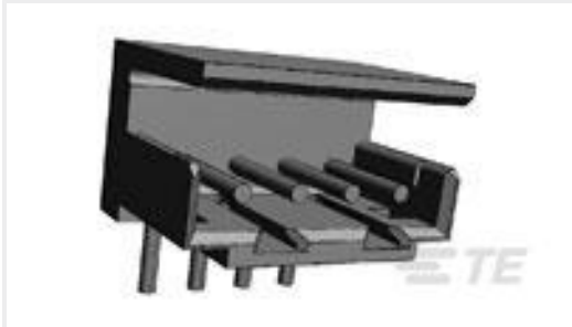
TE Part # 9-292260-1 CT P/HDR BOX H ASSY 11P T/P BL
