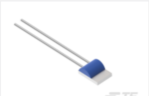
TE Part #NB-PTCO-160 Pt100, 2.0x2.3, Class B, PTFC101B1A0
