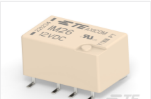
TE Part #3-1462039-1 IM26GR=IM RELAY 50mW 12V
