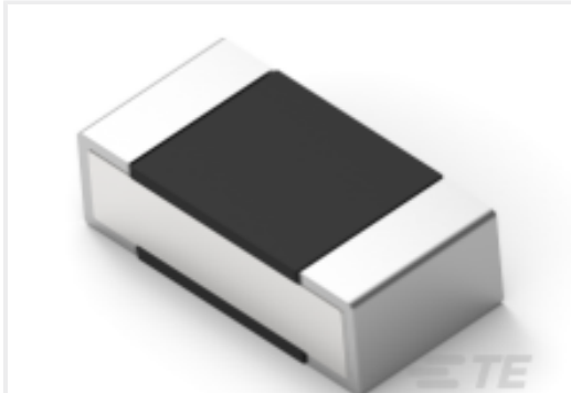
TE Part #5-2176304-1 RP 1E 0.1W 33R2 0.1% 25PPM 5K RL
