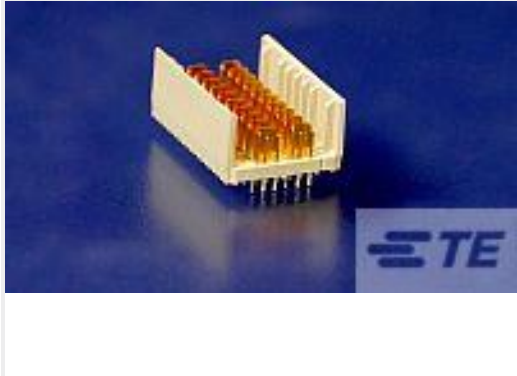
TE Part #1469734-1 HM-ZD 2PR HDR 40P SEQ, LF
