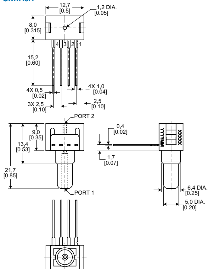
Figure 3. Mounting Dimensions (For Reference Only: mm/[in.]
