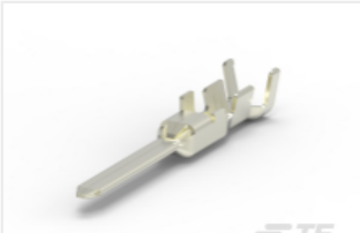
TE Part #2316817-3 HD3 TAB CONTACT AU0.38 L SIZE L/P
