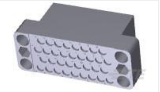
TE Part #201357-3 MALE BLOCK - 34 PL. SER. "M"
