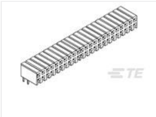
TE Part #1-2178615-0 RCPT,2MM,10P,R ANG MT,8AU,3.ST
