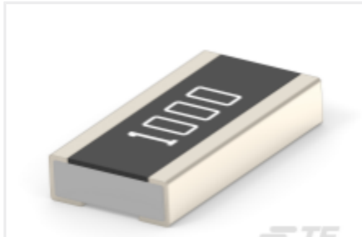
TE Part #7-2176558-2 3430 B2 1% 820R 100ppm 1k RL
