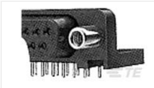
TE Part #788799-1 15 HTMSFL ASSY RA 318 (SL,BL)
