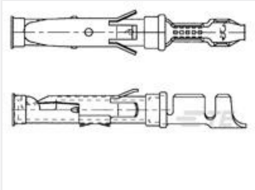
TE Part #163088-1 062 SOC.ASS. TYP3+
