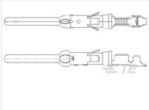
TE Part #163086-1 062 PIN ASS. TYP3+
