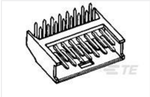
TE Part #280390-1 2X8P MODU II SHRD HDR, RT ANG, TIN
