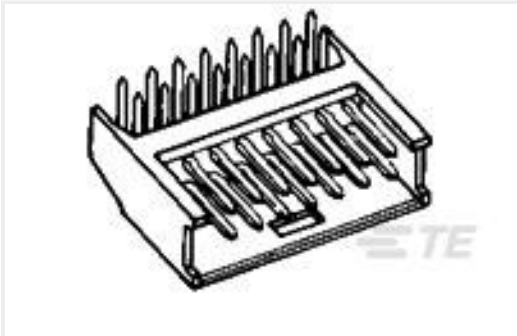
TE Part #280522-2 2X12P MODU II SHRD HDR, RT ANG, AU
