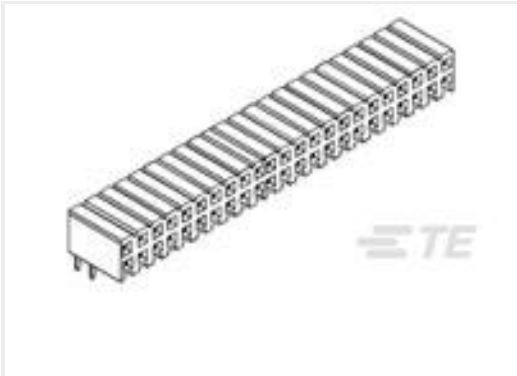
TE Part #2-1734531-2 RCPT,2MM,22P,R ANG MT,8AU,3.ST
