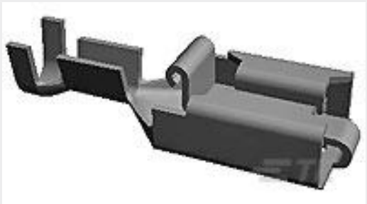
TE Part #928901-3 PL 250 REC TERMINAL 17-13 AWG TPBR LP
