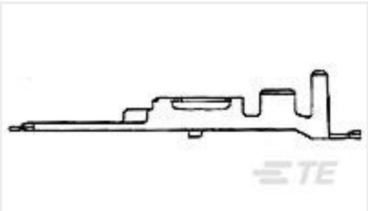
TE Part #172777-1 MIC MARE-2 TAB CONTACT
