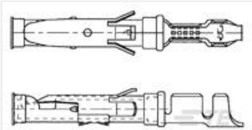
TE Part #1-163084-0 SPEC. PLATED
