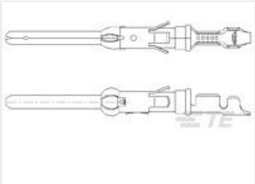
TE Part #163086-2 LOOSE PIECE PIN TYPEIII+ CONTACT SIZE 16
