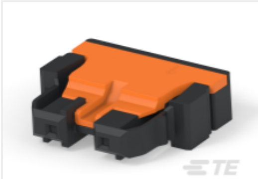
TE Part #524192-E SRCBUG A 6,20 * 2 CSI 206 E-HD ADVCOR TR
