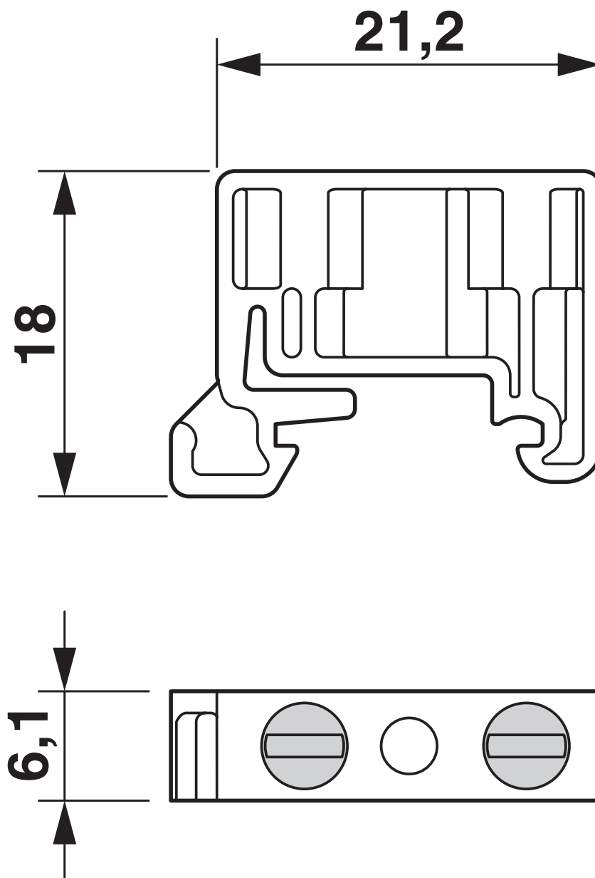
Dimensional drawing
