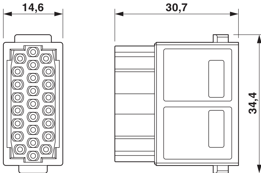
Dimensional drawing
